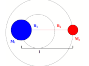
Figure 1: Rigid Rotor Model of a Diatomic Molecule
