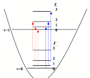
Figure 3: Rotation-Vibration Transitions
